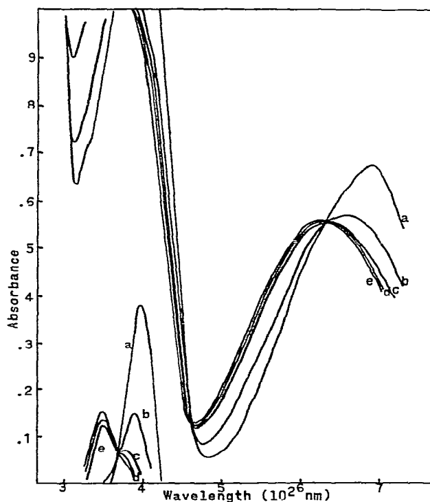
Fig 4 Spectrophotometric titration of 8.15 \times 10^{-5} M \text{Mo}(\text{phen})(\text{Ph}_3)_2(\text{CO})_2 in benzene with \text{GaMe}_3 . \text{GaMe}_3 concentration: (a) 0, (b) 2.77 \times 10^{-2} M , (c) 5.46 \times 10^{-2} M , (d) 9.34 \times 10^{-2} M , (e) 1.45 \times 10^{-1} M .
