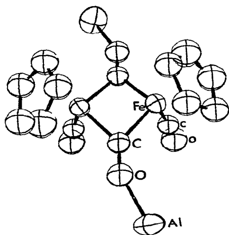
Fig 1 The structure of [\pi\text{-cp})\text{Fe}(\text{CO})(\text{COAlEt}_3)]_2 . Ethyl groups and hydrogen atoms have been omitted for clarity. (See ref 1)
